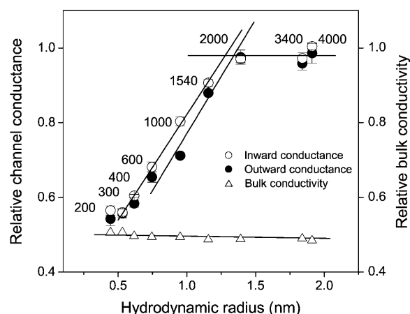
FIGURE 7 Relative changes in unitary maxi-anion single-channel conductances as a function of the hydrodynamic radii ( R ) of nonelectrolyte polymer molecules applied from both sides of membrane patches. The ascending straight line for channel inward conductances ( open circles ) is a linear fit to the data points for PEG 300–PEG 1540 and crosses the plateau level at R = 1.28 nm. The ascending straight line for outward conductances ( solid circles ) is a linear fit to the data points for PEG 600–PEG 2000 and crosses the plateau level at R = 1.34 nm. Relative decreases in the bulk conductivity of the polymer-containing control Ringer solutions used in these experiments ( open triangles ) are also plotted. Mean single-channel amplitudes at different voltages ( n = 5 –20 from at least five different patches) were used to construct I–V relationships and calculate slope conductances. Error bars represent standard errors of the linear fits.
